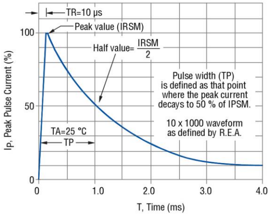
Figure 3 - Pulse Waveform
